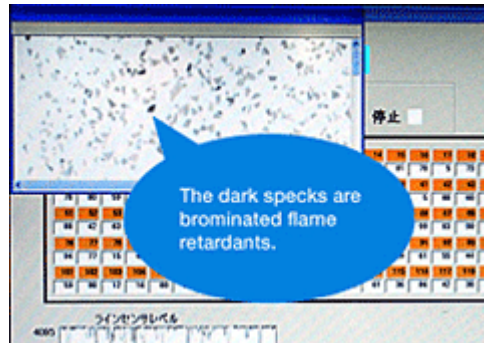
Award-winning technology where X-rays detect chips containing flame retardant in the granulated plastics mixture, and 124 individual air guns are instantly instructed to blow them aside.
